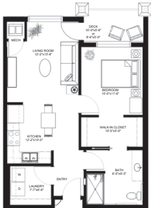
One Bedroom 660 Square Feet
