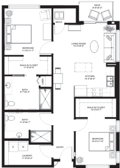
Two Bedroom, Two Bath 1,020 Square Feet
